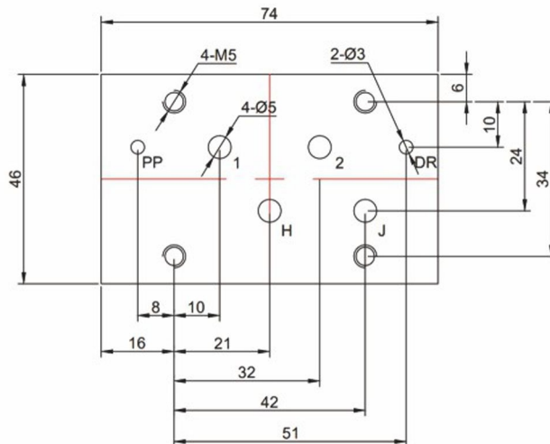
Fig. 2: HY602 Mechanical-hydraulic Servo Valve
